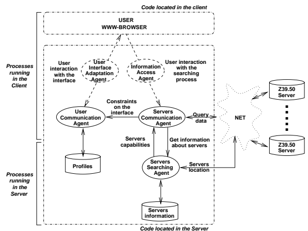
Figure 1: WAY-Z39.50 architecture
