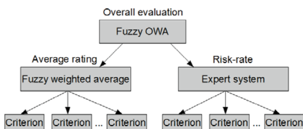
Figure 2: The simplified structure of the used goals tree
